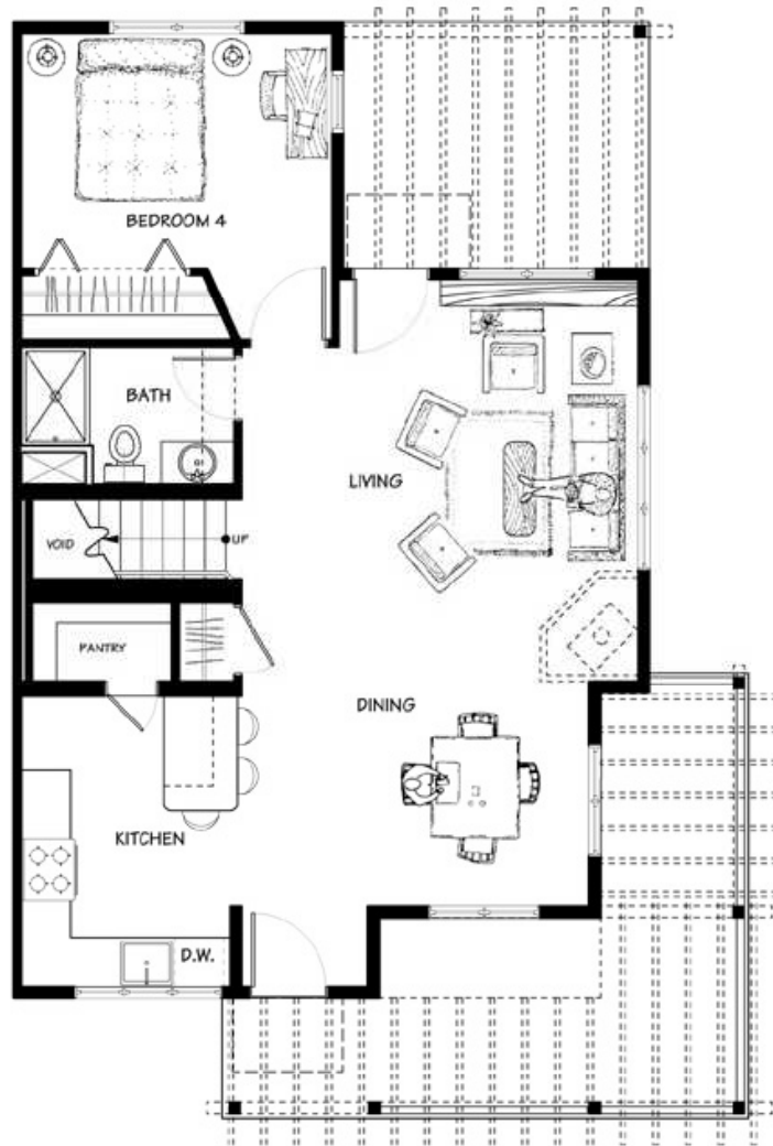
1 C UNIT 1ST FLOOR Scale: 3/16"=1'-0" UNIT SIZE: 1715 SQ.FT.
