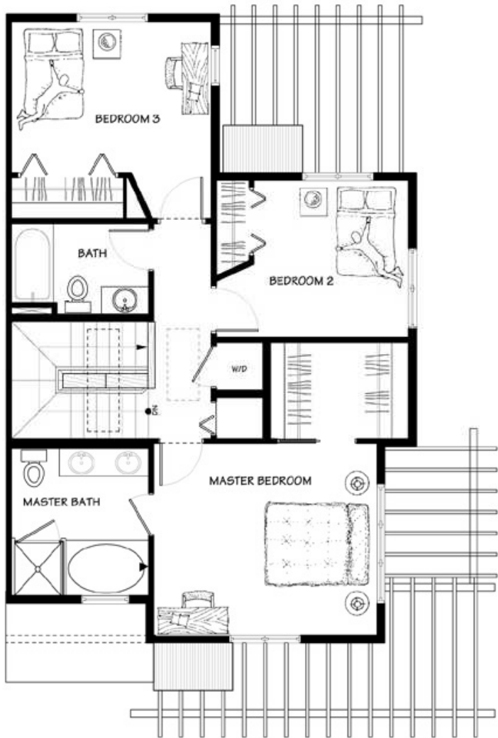
2 C UNIT 2ND FLOOR Scale: 3/16"=1'-0" UNIT SIZE: 1715 SQ.FT.
