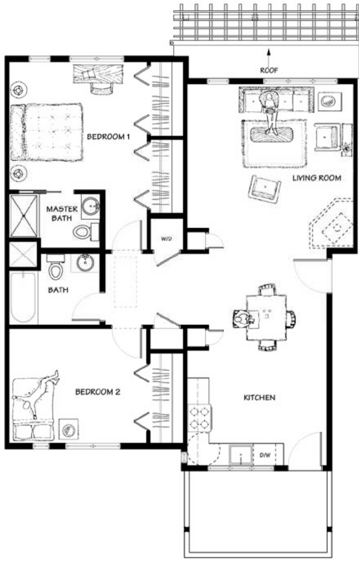
2 A2 UNIT 2ND FLOOR Scale: 3/16" = 1'-0" UNIT SIZE: 1092 SQ.FT.
